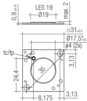
Dimensions in mm, *optical LES
